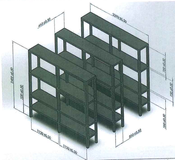
Figure 1: Three of five middle shelves. All five shelves should be anchored together at the top to prevent them from toppling over under load.
